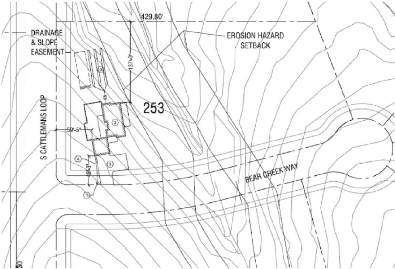
Site Plan 1" = 50'-0"
